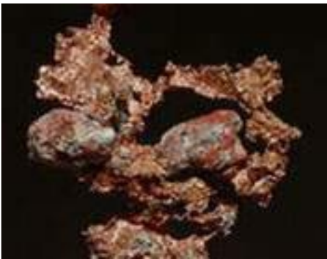
Native copper
